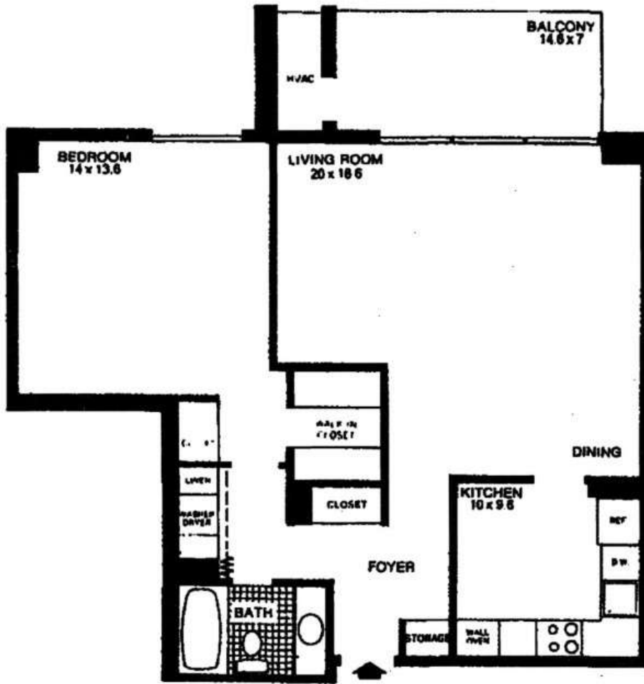
Type A 1 Bedroom 863 sqft.
